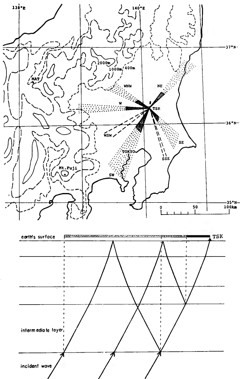
Fig. 11. The horizontal stretches swept by P-waves for five sets of the shock groups when it is assumed that a plane wave incident at the upper (shaded area) and lower (hatched area) interfaces of the intermediate layer is incident at TSK, and when a plane wave which is incident at the lower interface of the intermediate layer, reflects one time at the earth's surface and then reflects again at the lower interface (dotted area) of the intermediate layer, is incident at TSK, with the contour lines. The corresponding layered model and ray paths are shown in the lower half.
