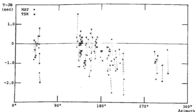
Fig. 14. Comparison of Jeffreys-Bullen travel-time residuals, observed minus computed ( T-J-B ) at TSK with those at MAT, as a function of azimuth. Residuals at these two stations for the same shocks which occurred from April, 1967 to December, 1968 are chained by dotted lines. Data were obtained from the USCGS earthquake data reports.
