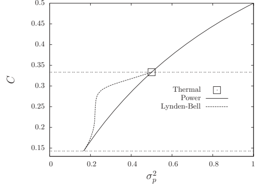
FIG. 4. Factor C as a function of momentum deviation at the critical point. The square point is for thermal equilibrium, the solid line is for power tails, and the broken line is for Lynden-Bell.
