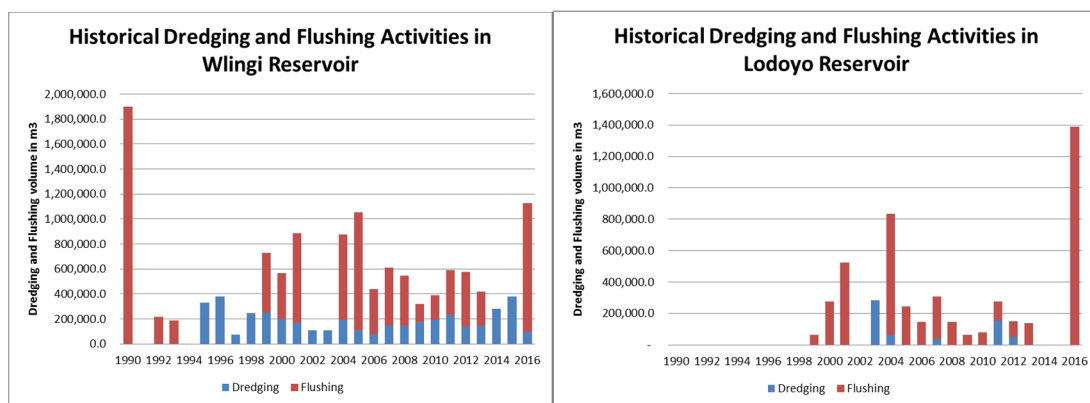
Fig. 2: Historical dredging and flushing activities in Wlingi reservoir (left) and Lodayo reservoir (right)
