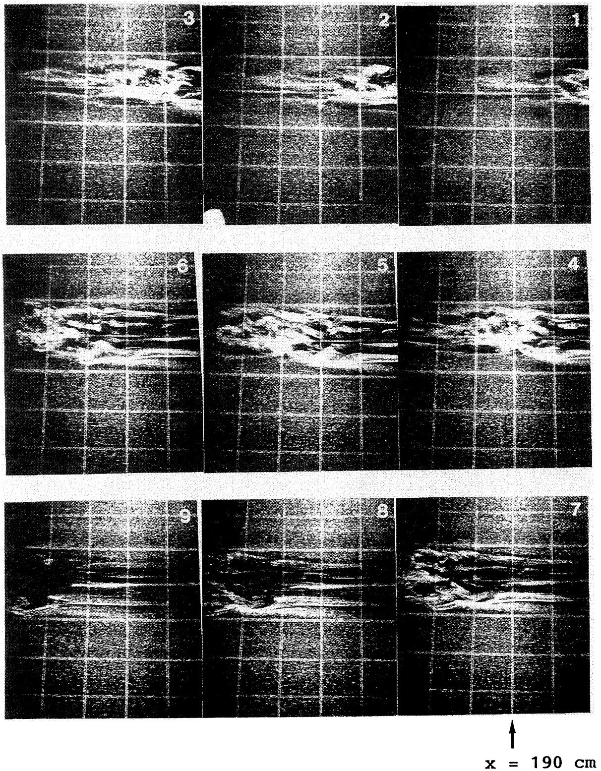
Fig. 7. Flow patterns of a turbulent spot on the plate surface, y = 0 \text{ mm} . x = 180 - 205 \text{ cm} . U_\infty = 10 \text{ cm/s} .
