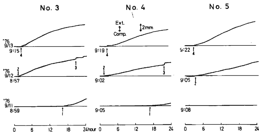
Fig. 19. Examples of the records of extensometers. Arrows show the onset time of displacement. The shown time are the starting time of the records.
