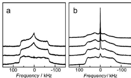
Figure 4. Variable-temperature solid-state ^2\text{H} NMR of (a) 1 and (b) 1' , both of which were synthesised using imidazole-D 4 . From bottom to top: 25 °C, 40 °C, 60 °C (for 1 and 1' ) and 80 °C (only for 1' ).
