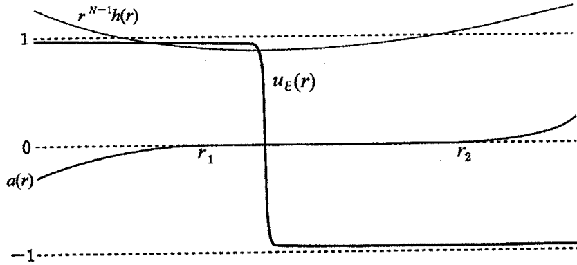
Fig 1: The profile of the global minimizer u_\varepsilon .
