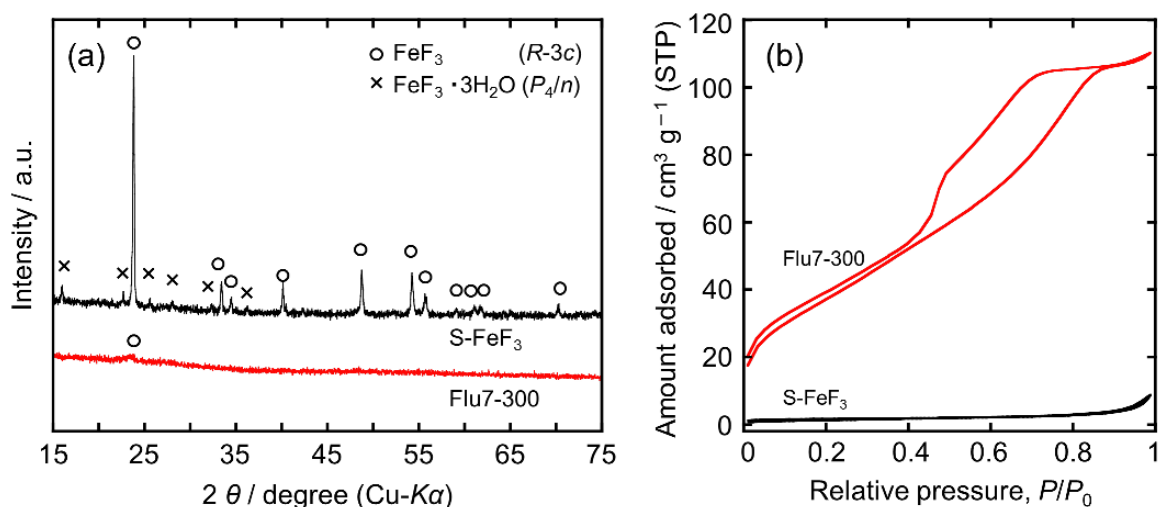
Fig. 6 (a) X-ray diffraction patterns and (b) nitrogen adsorption–desorption isotherms of the commercial \text{FeF}_3 (S- \text{FeF}_3 ) and the synthesized \text{FeF}_3 (Flu7-300).
