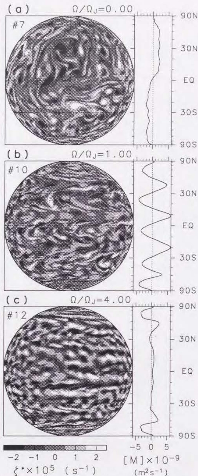
FIG. 10. Relative vorticity field for the disturbance components ( left ) and zonal mean zonal angular momentum ( right ) at t = 1000 J.days for the same three runs as in Figs.7 and 9. Map projection is the same as in Fig.1.
