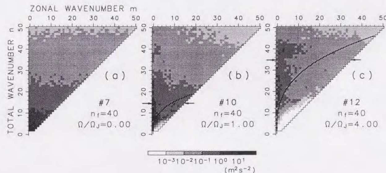
FIG. 11. Two-dimensional energy density averaged from 800 to 1000 J.days for the same three runs as in Figs.7, 9, and 10. Low-wavenumber region of 0 \leq m, n \leq 50 is shown. Thick arrows represent the wavenumber n_\beta . Solid curves indicate the “wave-turbulence boundary” at which the inverse of the vorticity advection time is comparable to the Rossby wave frequency.
