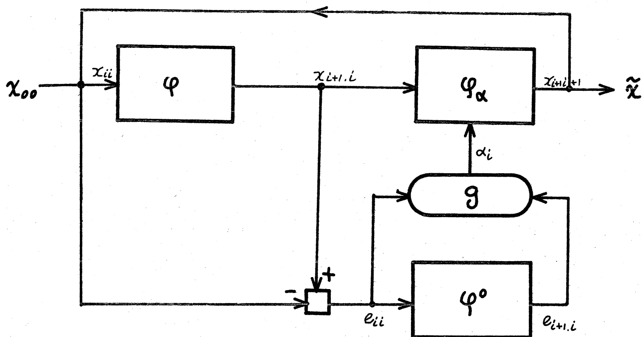
Fig. 3. Block Diagram of Algorithm (10).
