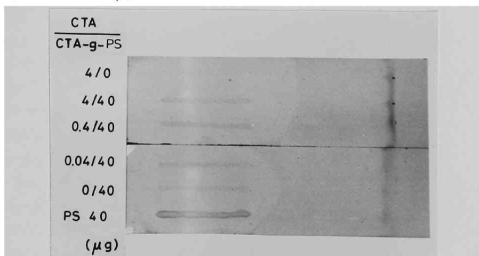
Fig. 6-8. Thin-layer chromatograms of the CTA homopolymer, the PS homopolymer, the isolated CTA-g-PS, and the CTA - CTA-g-PS mixtures with different mixing ratios (developer: methanol-methylene chloride(1 : 1) mixture).
