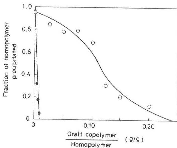
Fig. 7-3. An example of the protection effect of PVA-MMA graft copolymer on the precipitation of homoPMMA. The polymer precipitated was separated by simple decantation (●) or under centrifugation (O). (DP = 1,040).
