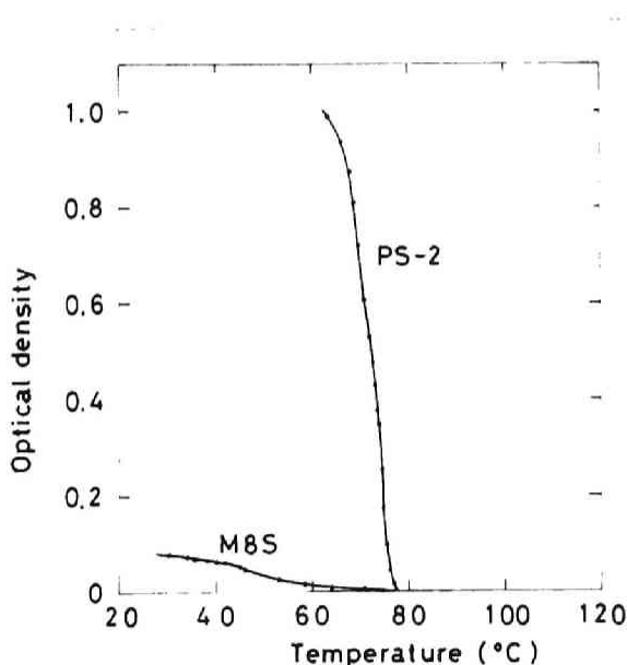
Fig. 9-1. Optical density-temperature curves of PVAC-styrene graft copolymer(M8S) and PS homopolymer(PS-2) in ethyl acetoacetate( c_{PS} \approx 5 mg/dl).
