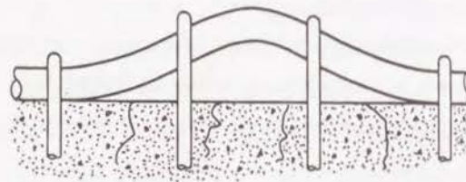
Fig.3-3 Buckling mode spanning three tie intervals [7]
