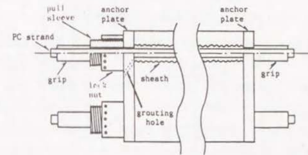
Fig.4-15 Dimensions of Series-E beams and details of its anchorage zone
