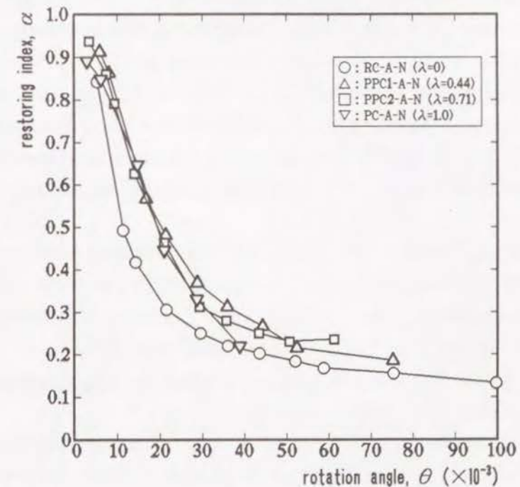
Fig.4-5 Elastic recovery expressed by restoring index (Series-A)
