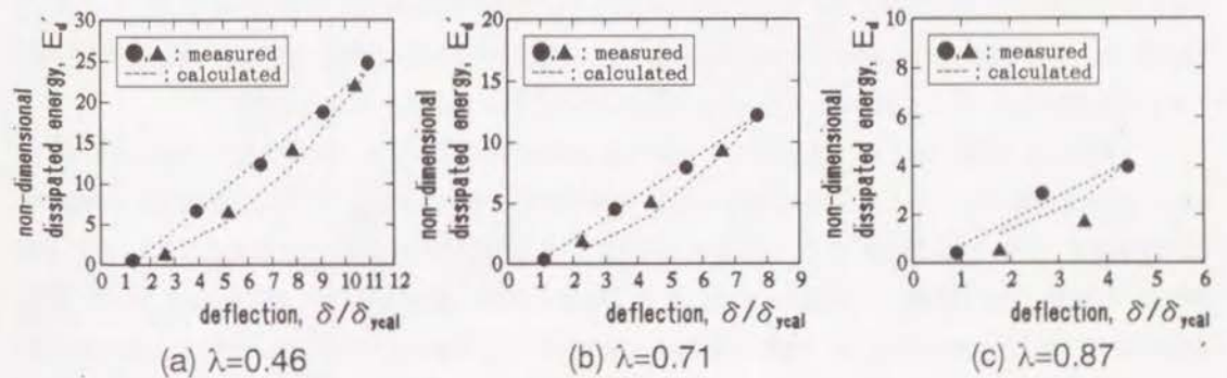
Fig.5-18 Examples of relationship between E_d' and \delta/\delta_{yca} of Series-C beams ( \rho_s=2.43\% )
