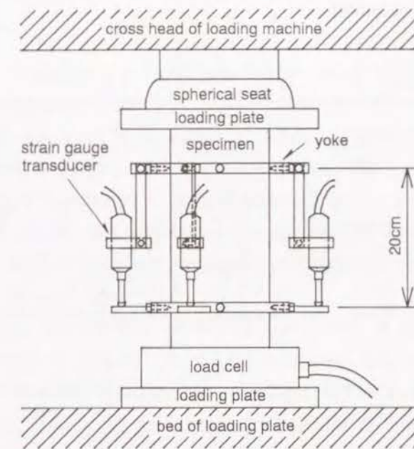
Fig.2-4 Loading and measuring apparatuses
