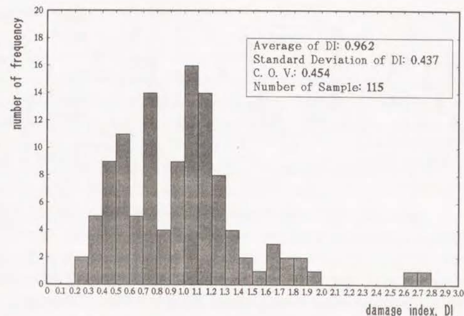
Fig.5-31 Statistics of DI at the ultimate state
