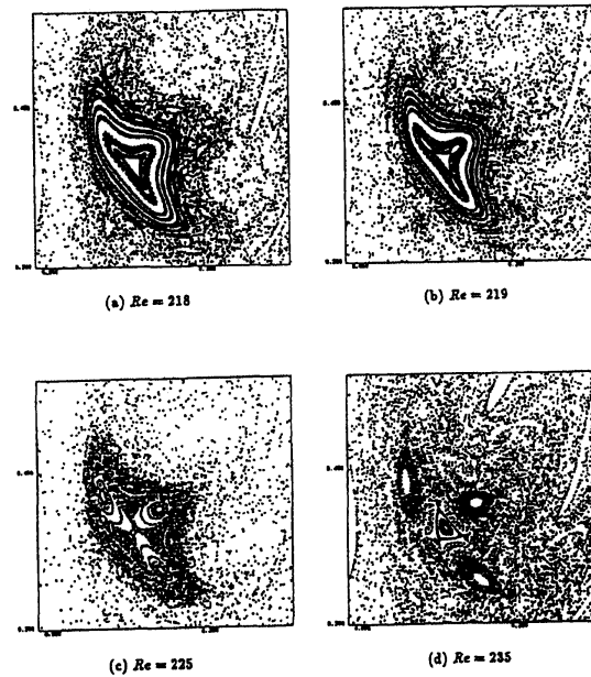
Figure 5. Poincaré sections near the 3 : 1 resonance (in the left lower quadrants).
