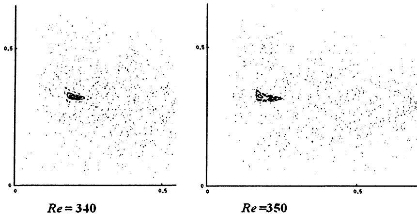
図 6 Poincaré sections near the 2:1 resonance
