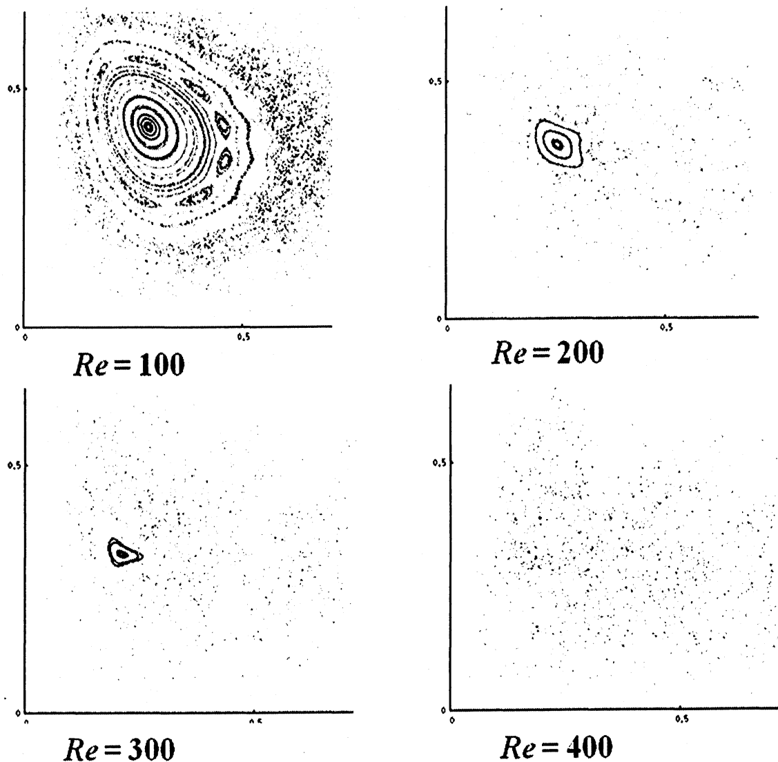
図 2 Poincaré sections for Re = 100, 200, 300 and 400
