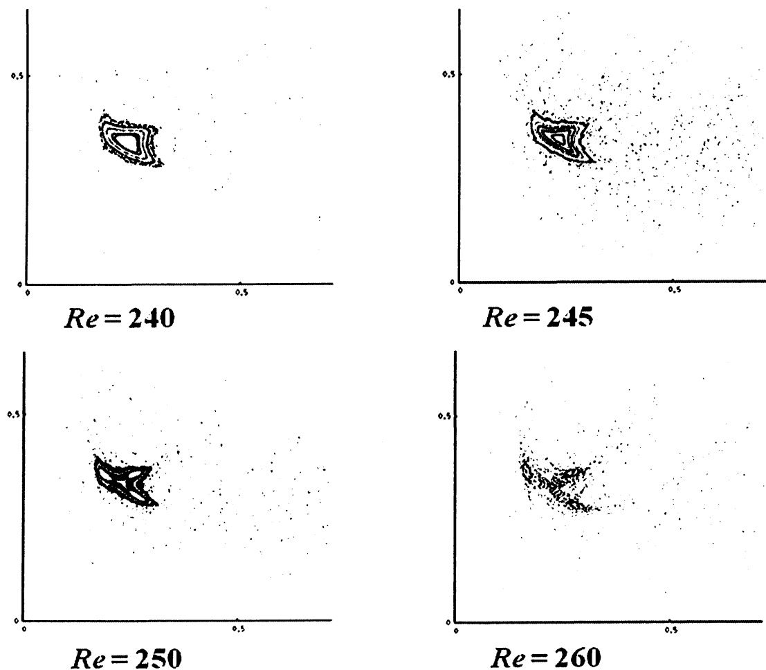
図 3 Poincaré sections near the 3:1 resonance
