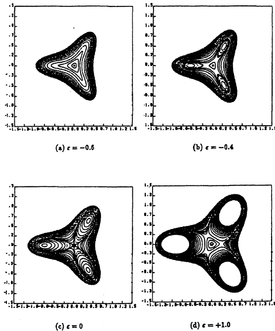
Figure 6. Phase portraits near the 3 : 1 resonance obtained by the normal form Hamiltonian H_3 for B = 1 and F = 1 .
