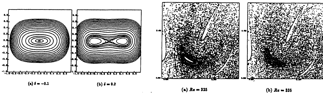
Figure 8. Phase portraits near the 2:1 resonance obtained by the normal form Hamiltonian H_2 for A = 1 and a = 1/4 .
