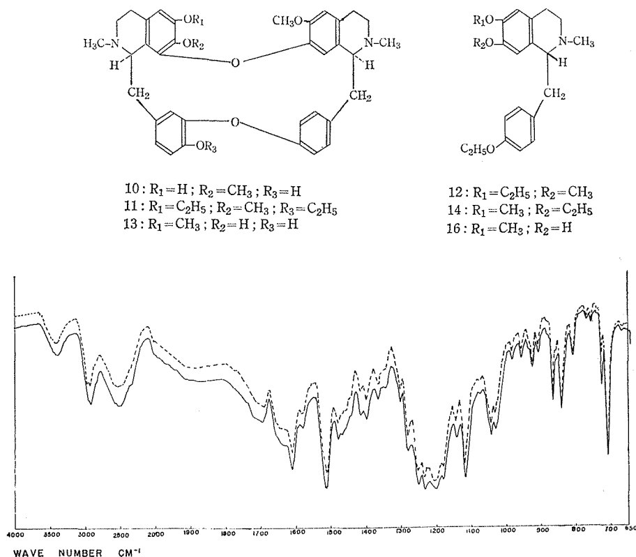
Fig. 4. I.R. Spectra (KBr) — Our Oxalate of Compound 14. ---- Ibuka's Sample of the Oxalate of Compound 14.
