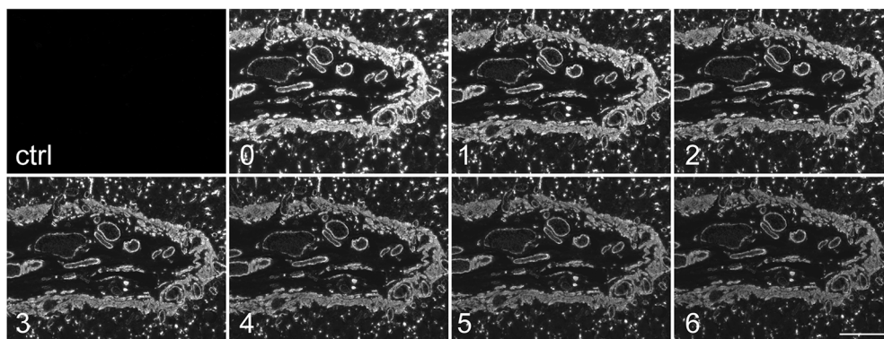
c SPiDER-βGal
