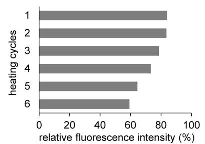
SPiDER-βGal
