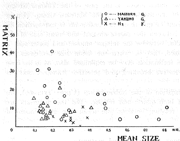
Fig. 5. Relation between amount of detrital matrix and mean size of sand grains.
