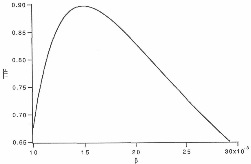
Fig. 4 Transit time factor (TTF) as a function of \beta for 34 MHz spiral resonator.
