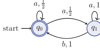
Figure 2: A probabilistic Büchi automaton \mathcal{P}
