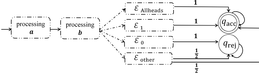
Figure 4: A schematic diagram of \mathcal{B}
