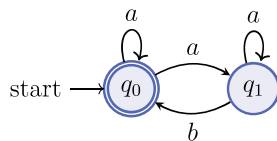
Figure 1: A non-deterministic Büchi automaton \mathcal{M}
