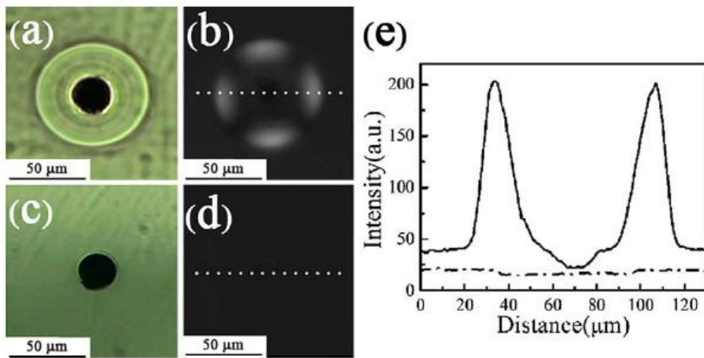
Fig. 1.9 Optical transmission image of the modification in the glass illuminated by natural light, and cross-polarized light, before((a) and (b)) and after heat treatment at 520 °C for 1h ((c) and (d)). (e) The transmitted light intensity along the white dotted line shown in (b) (solid curve) and (d) (dash and dot curve)
