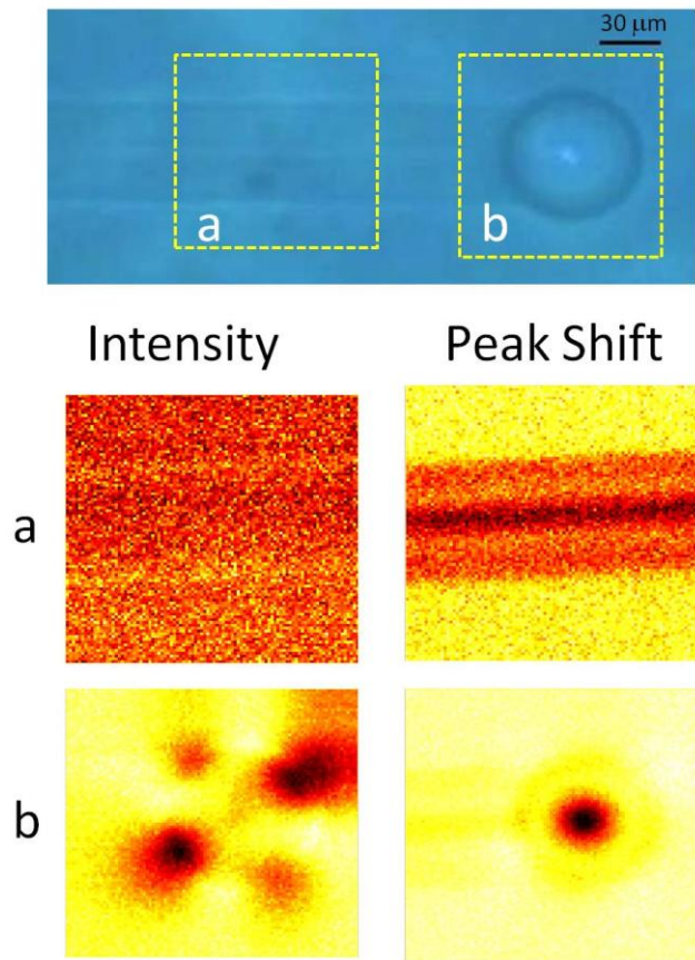
Fig. 2.7 Raman mapping of the area modified by femtosecond line-scan irradiation. (Scan speed: 100 \mu\text{m/s} , Laser power 350 mW)
