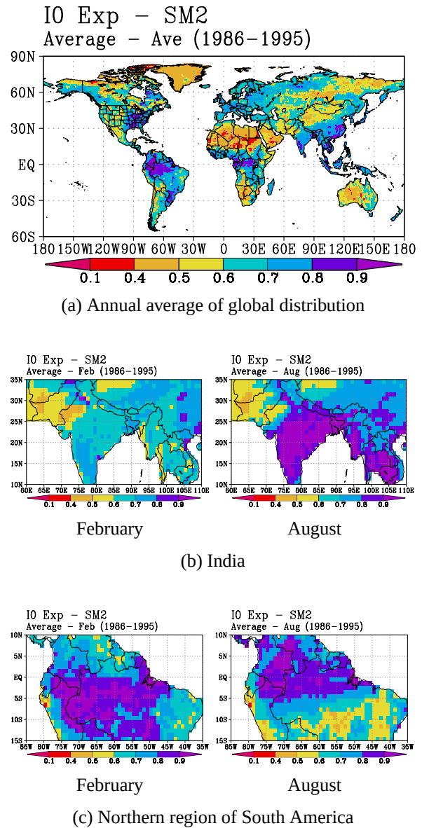
Fig. 5 A distribution of soil wetness at root zone, whose value shows average for 10 year by I0 exp.
