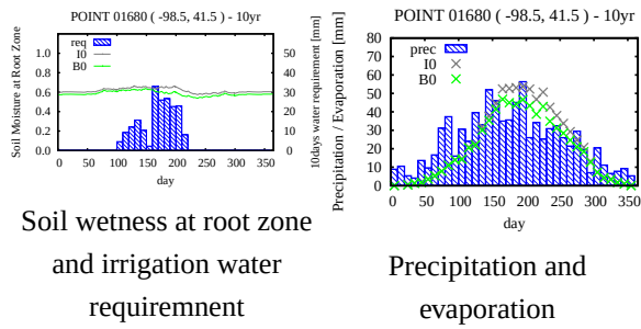
Fig. 8 10 years averaged annual cycle of hydrological variables at the point SNG (98.5W, 41.5N). The left axis means day of year and the vertical axis means hydrological value. Green line or mark shows the value estimated by B0 exp and black one shows the value of I0 exp.
