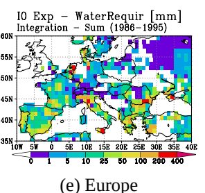
Fig. 7 A distribution of irrigation water requirement, whose value shows average for 10 year by I0 exp.
