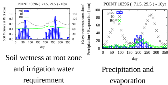
Fig. 9 10 years averaged annual cycle of hydrological variables at the point DBL (71.5E, 29.5N). The left axis means day of year and the vertical axis means hydrological value. Green line or mark shows the value estimated by B0 exp and black one shows the value of I0 exp.
