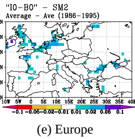
Fig. 6 The 10 years averaged distibutional difference of soil wetness at root zone between B0 exp and I0 exp.
