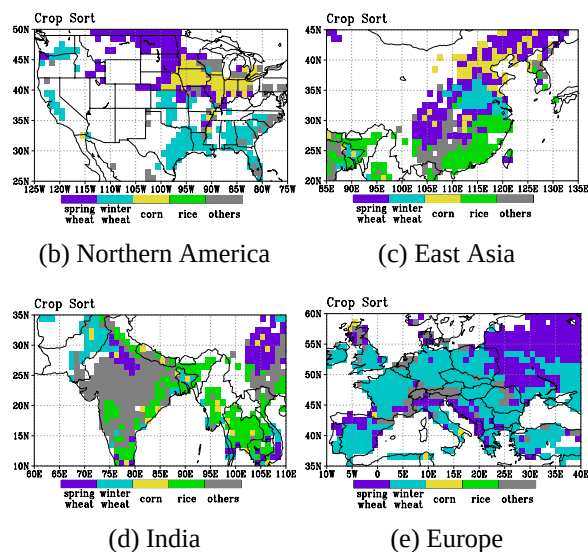
Fig. 2 Global map of crop type with 1-degree spatial resolution.
