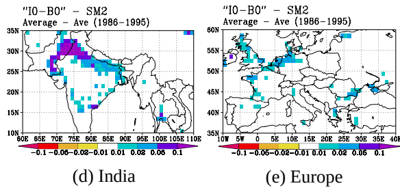
Fig. 6 The 10 years averaged distibutional difference of soil wetness at root zone between B0 exp and I0 exp.
