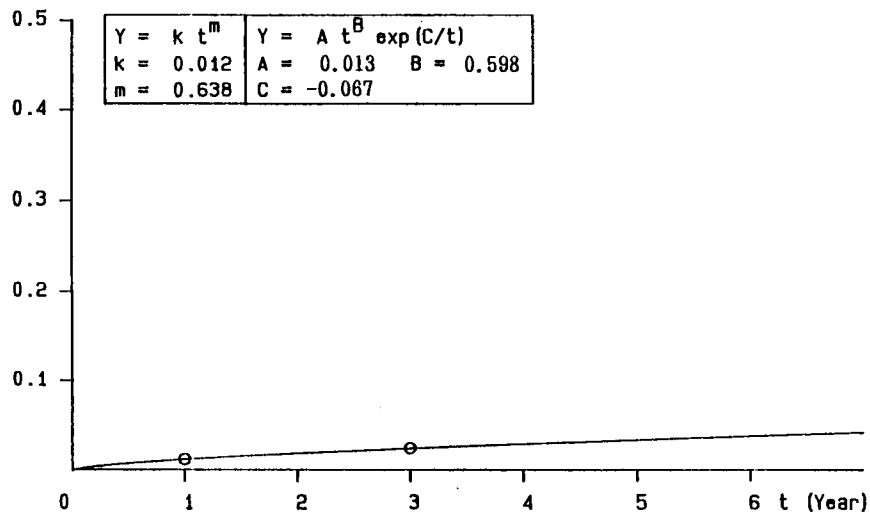
Fig. A1-U41 Long-term corrosion of bare steel underneath bridges Public Work Research Institute
