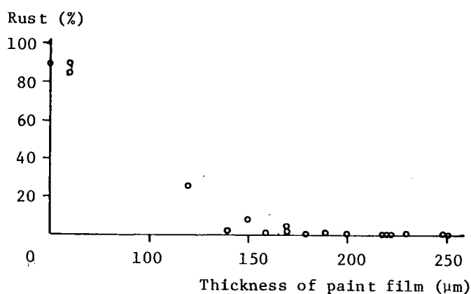
Fig. 3.1 Relation between minimum paint film thickness and the percent occurrence of rust at 2.5 year-exposure time 18)
