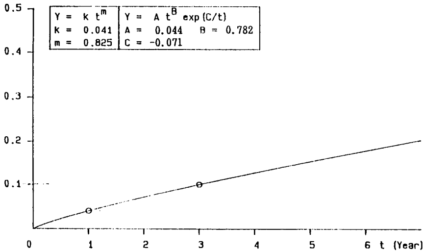
Fig. A1-U33 Long-term corrosion of bare steel underneath bridges Miyazaki
