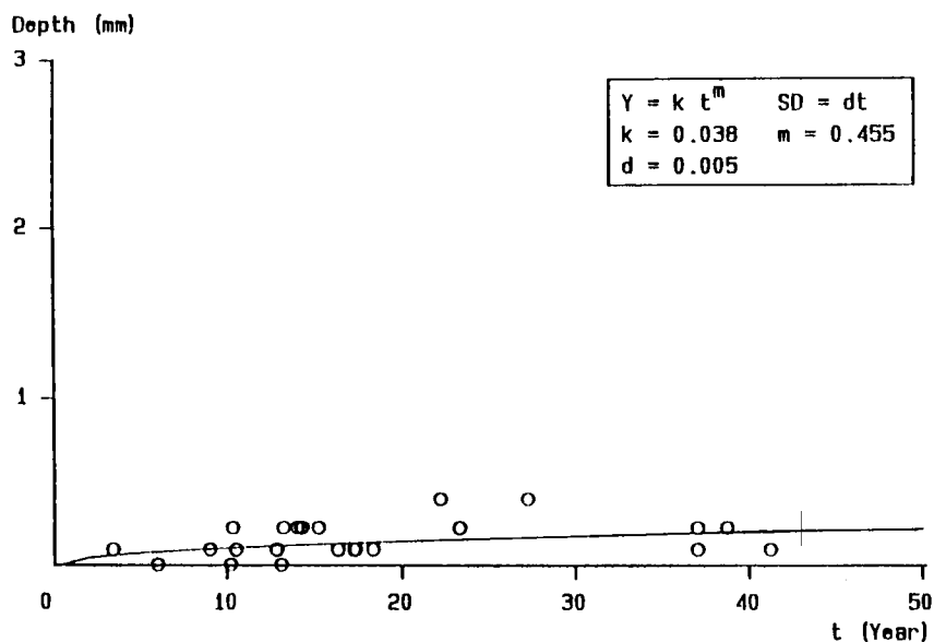
Fig. A4-4 Relation between corrosion depth and exposure time (Class 2) P4 End part of span of main girder (External girder) Web - Outer surface (City B, City envl.) Exposure time = accumulated time after paint life
