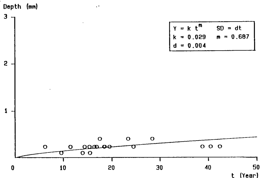
Fig. A4-3 Relation between corrosion depth and exposure time (Class 2) P3 End part of span of main girder (External girder) Lower surface of upper flange - Inner side (City B, City envl.) Exposure time = accumulated time after paint life
