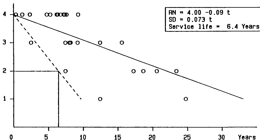
Fig. A2-21 Relation between RN of paint film deterioration and exposure time P23 Middle part of span of main girder (Internal girder) Lower surface of upper flange (City A, Rural envi.) Paint type = Alkyd resins (N=29)
