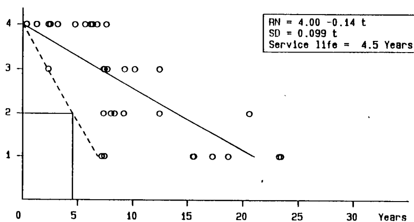
Fig. A2-20 Relation between RN of paint film deterioration and exposure time P21 Middle part of span of main girder (External girder) Lower surface of lower flange (City A, Rural envl.) Paint type = Alkyd resins (N=33)
