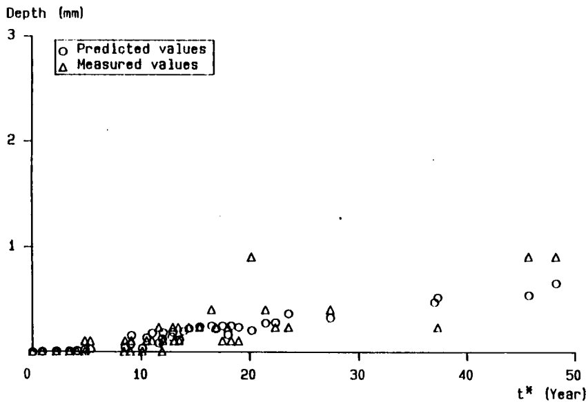
Fig. A5-17 Relation between corrosion depth and exposure time P17 Middle part of span of main girder (External girder) Web - Outer surface (Rural and city envi.) Exposure time = accumulated time after paint life
