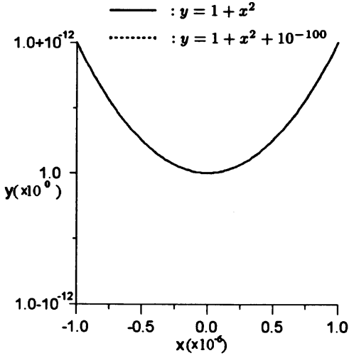
(a) Magnification: 10^6 in x , 10^{12} in y .
