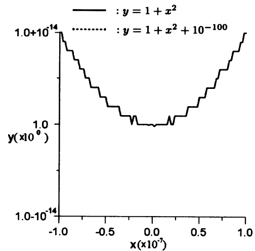
(b) Magnification: 10^7 in x , 10^{14} in y .
