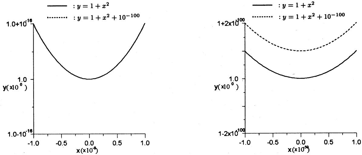
(a) Magnification: 10^8 in x , 10^{16} in y .
