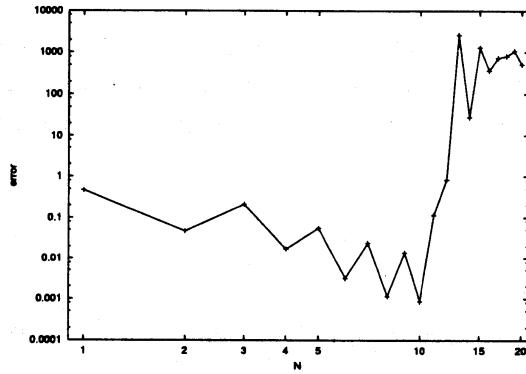
(a) Double precision
