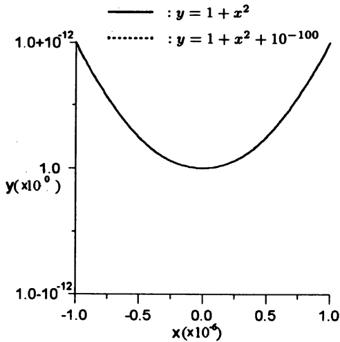
(a) Magnification: 10^6 in x , 10^{12} in y .
