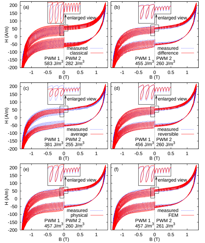
Fig. 5. Simulated B-H loops for 2 types of PWM waveforms where measured iron losses per cycle are 458 and 252 J/m 3 : (a) classical eddy-current theory, (b) standard Cauer circuit with finite-difference approximation (21) with \varepsilon = 1 , (c) standard Cauer circuit with average approximation H_{ave} , and (d) the reversible component H_{rev} are used to represent the second inductor L/5 . For comparison, Fig. 5(e) and (f) shows the B-H loops given by the physical Cauer circuit shown in Fig. 3(b) and the one-dimensional finite element eddy-current analysis along the z -direction with 10 first-order elements.
