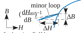
Fig. 4. Permeability for the minor B-H loop.
