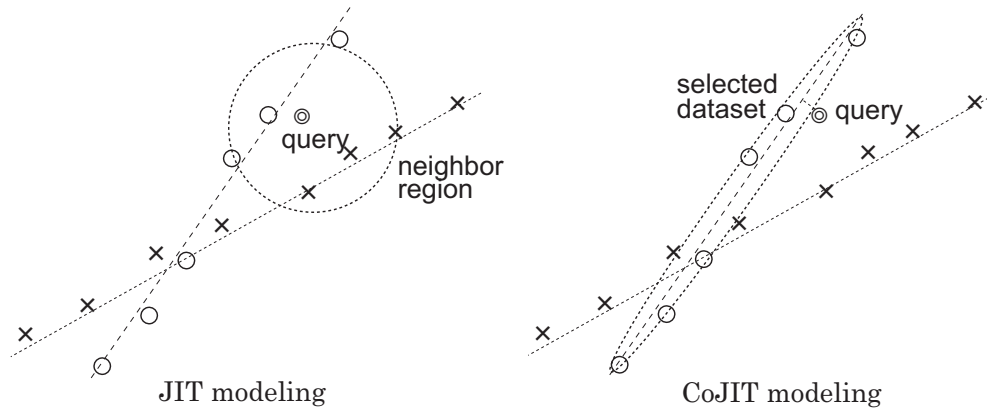
Figure 3: Sample selection in JIT modeling (left) and CoJIT modeling (right)
