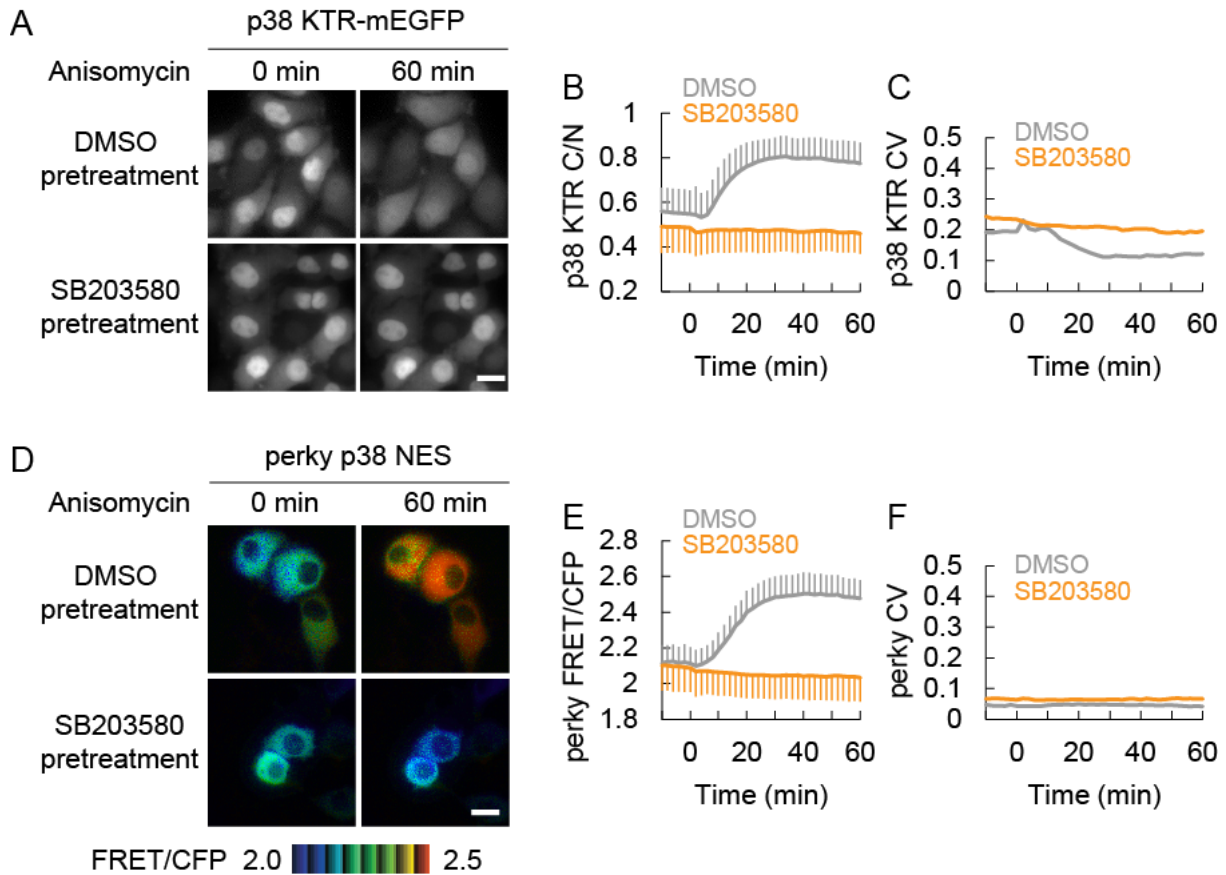
Figure 18. Cell-to-cell variability in p38 signaling.
