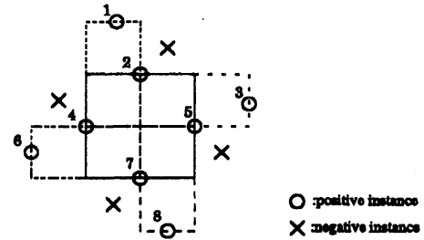
Figure 3: Example of the case that a concept is possibly found after the for-loop in which no concept is found.
