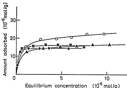
Fig. 6 Dependence of DH of PVAc on the adsorption from benzene onto preswollen wood meal in the range of high DH. ○: 0% DH, ▲: 21.8% DH, ■: 25.7% DH, ◆: 29.4% DH, ●: 30.4% DH.
