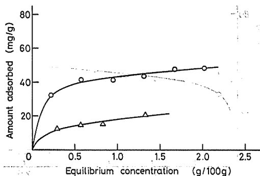
Fig. 1 Adsorption isotherms of PVAc 25 (○) and PVAc 300 (△) from benzene on preswollen wood meal.
