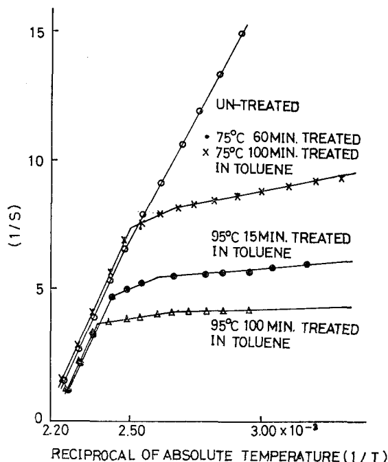
Fig. 1. Relation between the reciprocal relative shrinkage 1/S and the reciprocal temperature 1/T for polypropylene fibers treated in toluene.
