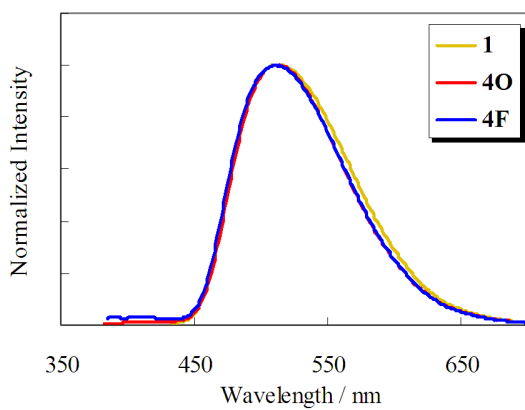
Figure 3. Normalized emission spectra of polymers and model compound in \text{CHCl}_3 ( 1.0 \times 10^{-5} \text{ M} ).
