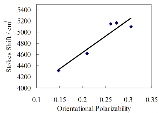
Figure 4. Lippert plot of model compound 1 .
