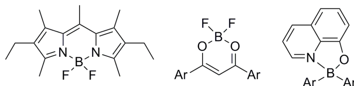
Figure 3. Examples of BODIPYs (left), boron diketonate (centre) and boron quinolate (right).
