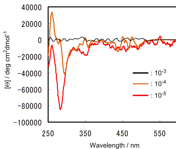
Figure 3. Concentration dependence in \text{CHCl}_3 of CD spectrum of poly1 .
