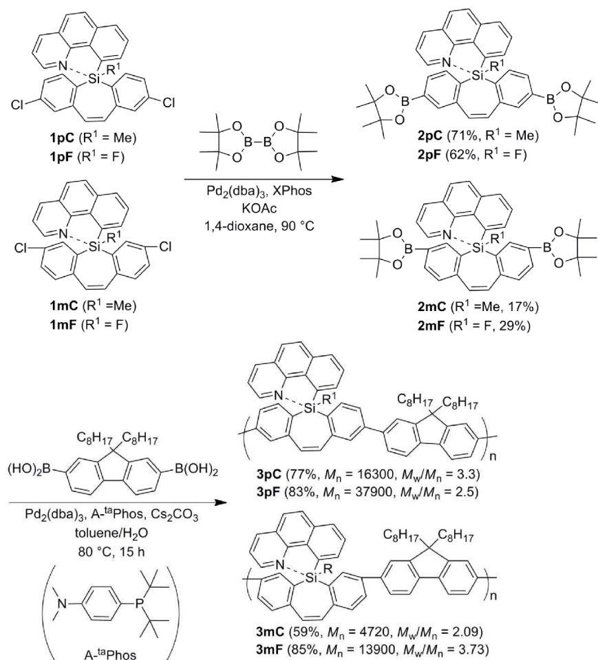
Scheme 1. Synthesis of polymers
