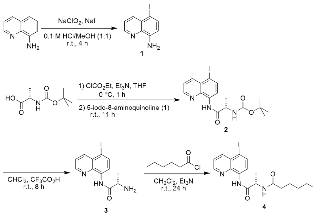
Scheme 1. Synthesis of N -hexanoyl-L-alanine- N' -5-iodo-8-quinolylamide
