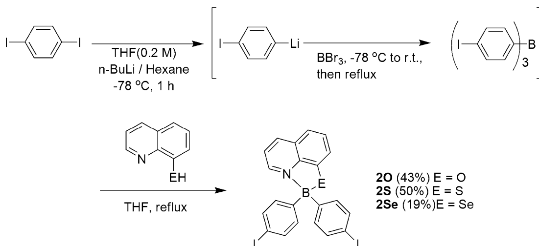
Scheme 2. Synthesis of monomers 2O , 2S , and 2Se .
