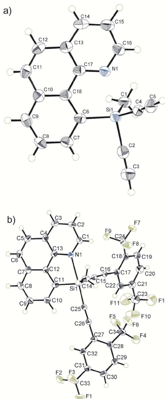
Figure 1. The X-ray crystal structures of a) 1E and b) 2F with thermal ellipsoids drawn to the 50% probability level. Selected bond lengths [ \text{\AA} ] and angles[ ^\circ ]: 1E : Si1–N1 2.434, C1–Si1–C4 116.5(2), C4–Si1–C6 114.12(19), C1–Si1–C6 119.48(18), C2–Si1–C4 101.03(18), C1–Si1–C2 99.25(19), C2–Si1–C6 101.52(18); 2F : Si1–N1 2.3454(17), C15–Si1–C14 113.8(11), C15–Si1–C11 117.9(9), C14–Si1–C11 122.4(11), C15–Si1–C25 95.8(10).
