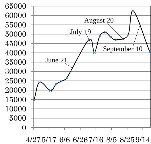
Fig.12 Discharge in 2008 monsoon at Bahadurabad
