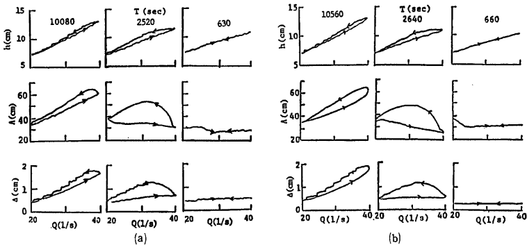
Fig. 7 Simulated hystereses of dune height, dune length and mean flow depth. (a) : for triangular hydrographs. (b) : for sinusoidal hydrographs.
