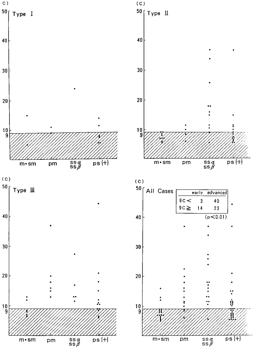
Fig. 3 Comparisons of the highest DNA ploidy values of the original tumors among groups of m*sm, pm, ssα*ssβ and ps (+) in relation to their nuclear DNA modal patterns in Type I, II, III and All cases. Shaded area indicates the highest DNA ploidy values below 9C, within which differences in the highest DNA ploidy values among m*sm, pm, ssα*ssβ and ps (+) were nonsignificant ( p > 0.05 ). Statistical difference ( p < 0.01 ) by Fisher's exact test (early vs. advanced in All cases). Statistical difference ( p < 0.01 ) by Fisher's exact test (ssα*ssβ vs. ps (+) in All cases).
