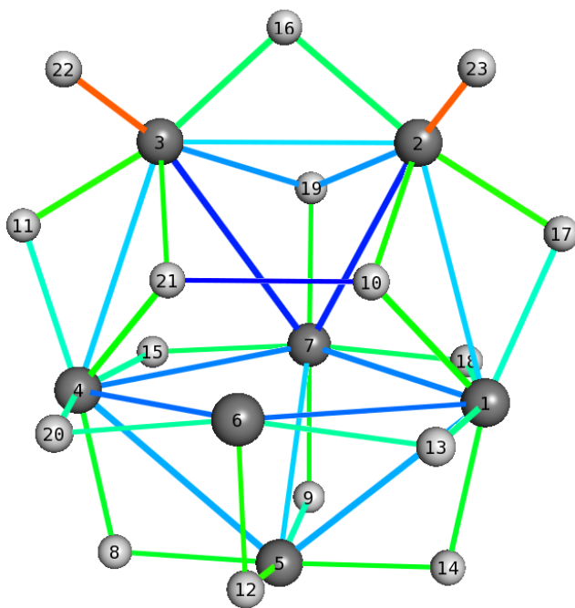
(f) \text{Pd}_7\text{H}_{16}
