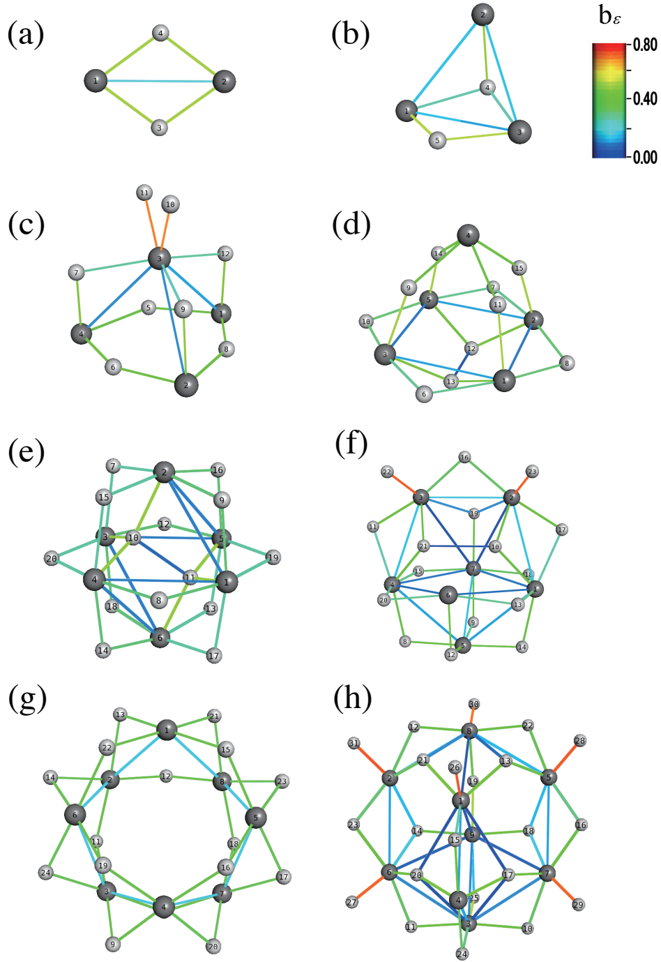
Figure 1: Optimized structures and bond order for hydrogenated Pd clusters: (a) \text{Pd}_2\text{H}_2 , (b) \text{Pd}_3\text{H}_2 , (c) \text{Pd}_4\text{H}_8 , (d) \text{Pd}_5\text{H}_{10} , (e) \text{Pd}_6\text{H}_{14} , (f) \text{Pd}_7\text{H}_{16} , (g) \text{Pd}_8\text{H}_{16} and (h) \text{Pd}_9\text{H}_{22} . The bonds are drawn at which Lagrange points are found and our energy density based bond order b_\epsilon (eq. (5)) is shown by color.
