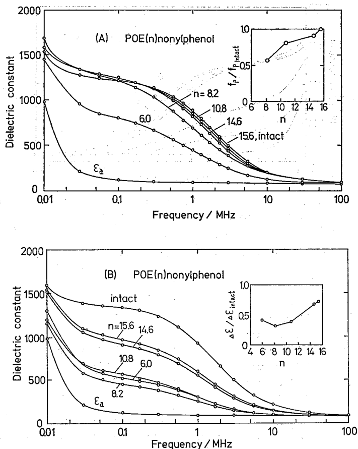
Fig. 13. Effect of POE chain length n on dielectric dispersion in the absence (A) and in the presence of 1 M sorbitol (B). The concentrations of the detergents are 1 mM (A) and 0.5 mM (B). The relative characteristic frequency f_p/f_{p, \text{intact}} (A) and the relative magnitude \Delta\epsilon/\Delta\epsilon_{\text{intact}} (B) of dielectric dispersion are depicted in the figures.
