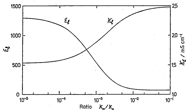
Fig. 22. Effect of change in \kappa_m on \epsilon_i and \kappa_i . The calculation is carried out by Pauly-Schwan's equation. Volume fraction and diameter of cells are 0.3 and 3.8 \mu\text{m} , respectively, through the calculation. Other parameters are the same as those in Fig. 21.
