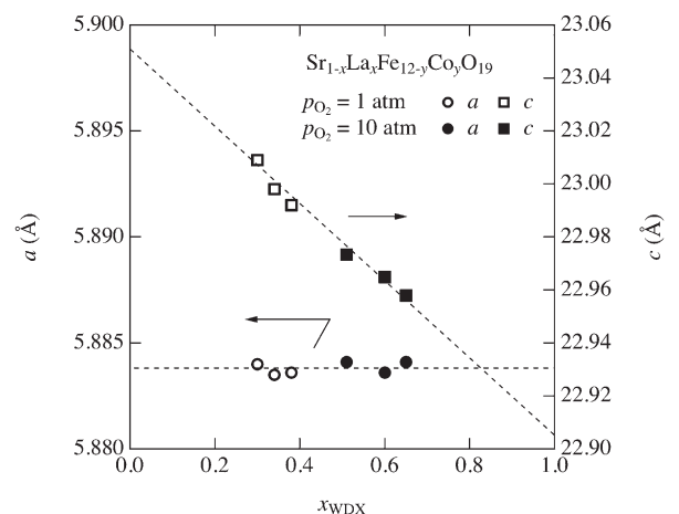
Fig. 5 Lattice constants for \text{Sr}_{1-x}\text{La}_x\text{Fe}_{12-y}\text{Co}_y\text{O}_{19} plotted against La concentration determined by WDX analysis. Dashed lines are guide for eyes.
