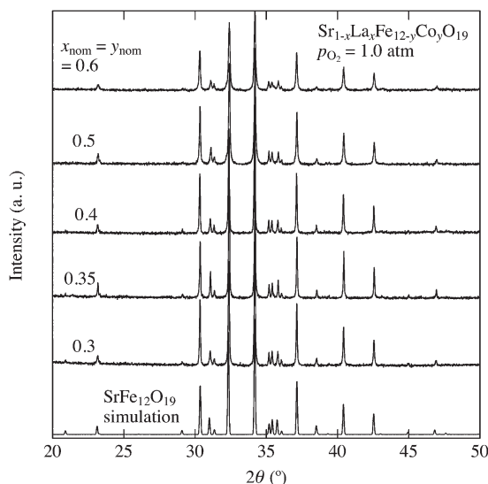
Fig. 3 XRD patterns for \text{Sr}_{1-x}\text{La}_x\text{Fe}_{12-y}\text{Co}_y\text{O}_{19} with x_{\text{nom}} = y_{\text{nom}} fired at p_{\text{O}_2} = 1.0 \text{ atm} . Apparent secondary phases other than the M-type ferrite were not observed in all composition range.
