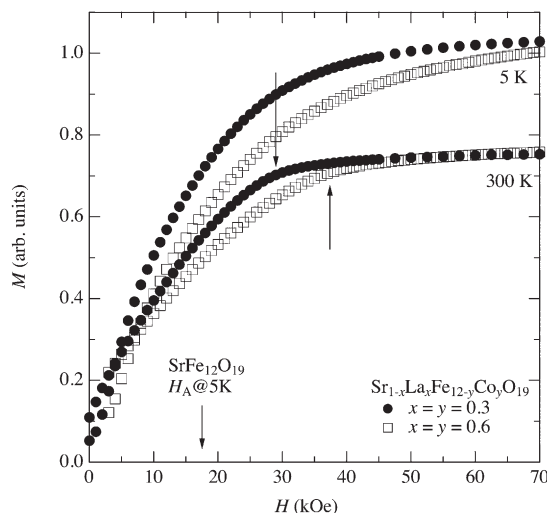
Fig. 7 Hard axis magnetization for \text{Sr}_{1-x}\text{La}_x\text{Fe}_{12-y}\text{Co}_y\text{O}_{19} with x = y = 0.3 and 0.6 at T = 5 and 300 \text{ K} .
