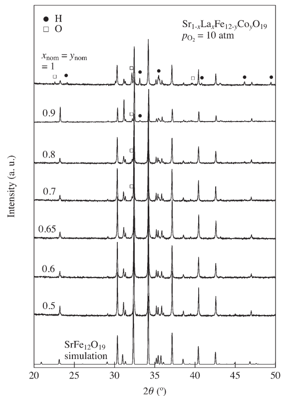
Fig. 4 XRD patterns for \text{Sr}_{1-x}\text{La}_x\text{Fe}_{12-y}\text{Co}_y\text{O}_{19} with x_{\text{nom}} = y_{\text{nom}} fired at p_{\text{O}_2} = 10 \text{ atm} .
