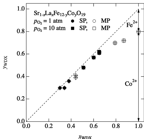
Fig. 6 La ( x ) and Co ( y ) compositions determined by WDX for the cases with x_{\text{nom}} = y_{\text{nom}} . Dashed line represents the relation of x = y . SP and MP represent single-phase and multi-phase samples judged from XRD patterns, respectively. Points below the dashed line indicate the presence of \text{Fe}^{2+} appeared to compensate the extra-charge due to the substitution of \text{La}^{3+} for \text{Sr}^{2+} .
