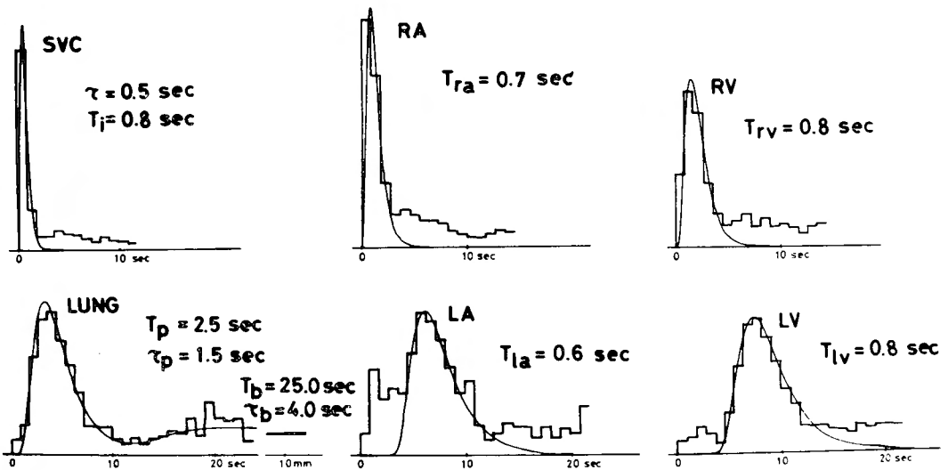
Fig. 14. Simulation results of a normal subject (32y. male). Total Blood Volume : 5.7 \text{ L} , Cardiac Index : 5.27 \text{ L/min/m}^2 , Mean Volumes (Transit Times) of Cardiac Chambers, Lung and Body : RA = 62 \text{ ml/m}^2 (0.7 sec), RV = 70 \text{ ml/m}^2 (0.8 sec), Lung = 350 \text{ ml/m}^2 (4.0 sec), LA = 53 \text{ ml/m}^2 (0.6 sec), LV = 70 \text{ ml/m}^2 (0.8 sec), Body = 2.250 \text{ ml/m}^2 (29.0 sec).
