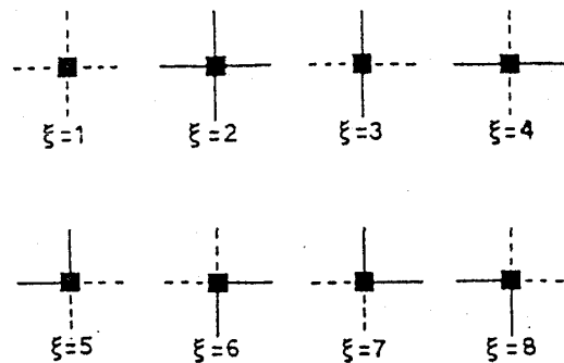
Fig. 3. Vertex configurations \xi_{k,l,v} which are permitted in the eight-vertex model.
