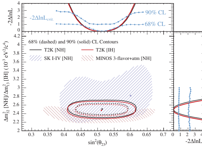
FIG. 3 (color). The 68% and 90% C.L. confidence regions for \sin^2(\theta_{23}) and \Delta m^2_{32} (NH) or \Delta m^2_{13} (IH). The SK [49] and MINOS [7] 90% C.L. regions for NH are shown for comparison. T2K's 1D profile likelihoods for each oscillation parameter separately are also shown at the top and right overlaid with light blue lines and points representing the 1D -2\Delta \ln \mathcal{L}_{\text{critical}} values for NH at 68% and 90% C.L.
