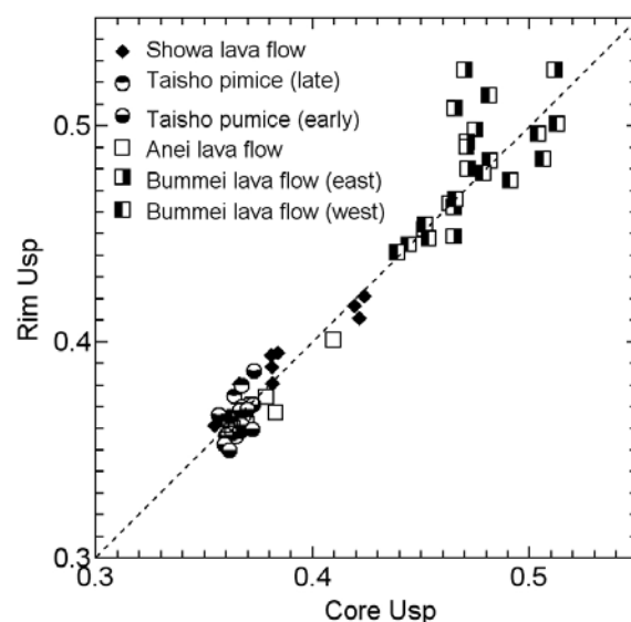
Fig. 2 Core and rim compositions of the magnetite phenocrysts in the pumices of Taisho eruption and lava flows of the three historical eruptions.
