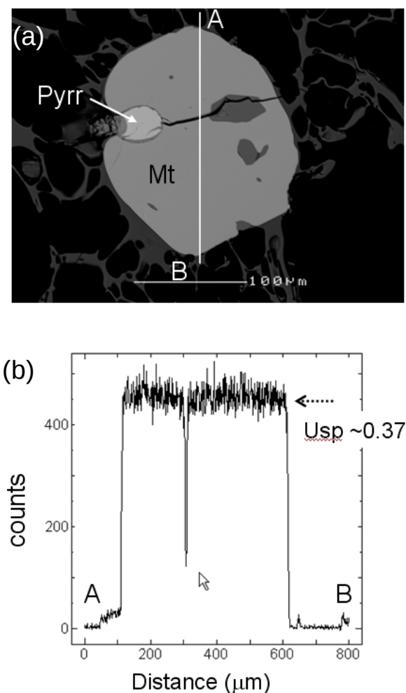
Fig. 1 (a) Backscattered electron image of representative magnetite phenocryst ("Mt") in the pumice of Taisho eruption. "Pyrr" represents pyrrhotite inclusion. (b) Line profile of the titanium K\alpha X-ray count along the traverse A-B in (a). The magnetite phenocryst has a homogeneous Ti concentration corresponding to the ulvöspinel content (Usp) of 0.37. See text for the detailed analytical conditions.
