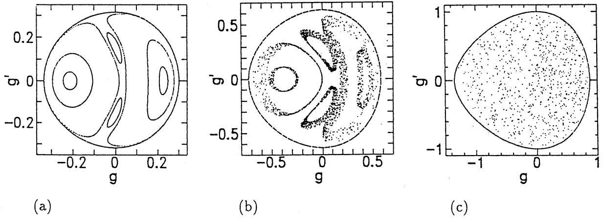
Figure 4: Surface of section for the non-integrable case \alpha = \beta , where \alpha = \beta = 1/3, \lambda = 2 and V = 1/2 : (a) E=0.005 , (b) E=0.2 , (c) E=0.5 .
