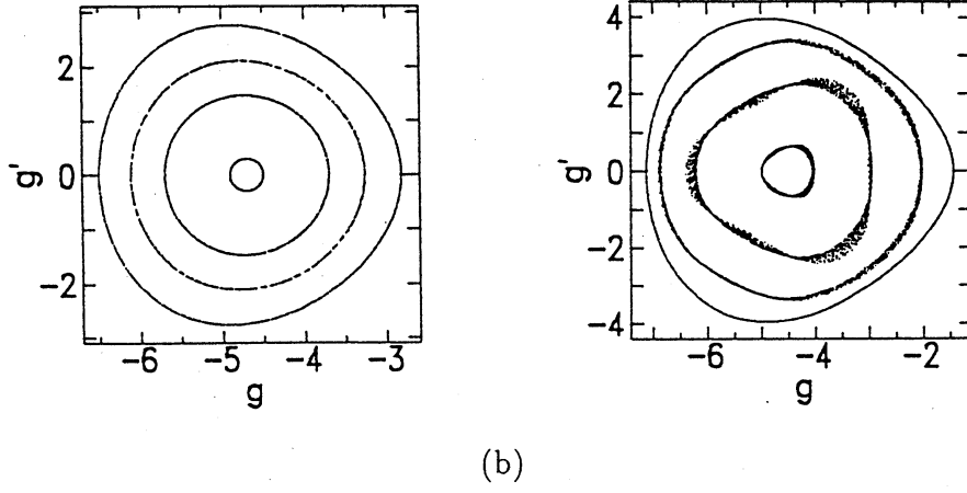
Figure 3: Surface of section for the non-integrable case \alpha = -\beta when V - \lambda/2 + 2/\beta \neq 0 , where \alpha = -1/3, \beta = 1/3, \lambda = 2 and V = 1/2 : (a) E=3.79 , (b) E=7.79 .
