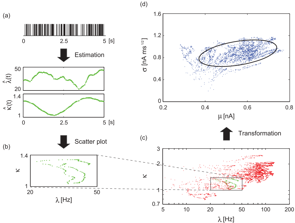
FIG. 6. (Color online) Analyzing in vivo data using the transformation method. (a) MAP estimates of the firing rate \hat{\lambda}(t) and irregularity \hat{\kappa}(t) for a spike sequence in a single trial. (b) Scatter plot of the estimated firing characteristics for each spike in a log-log (\lambda, \kappa) plane. (c) Scatter plot of the log-log data (\lambda, \kappa) for a single neuron within and across trials. (d) Scatter plot of the estimated input mean and fluctuation (\hat{\mu}, \hat{\sigma}) . Ellipses represent 75% quantiles of two-dimensional Gaussian distribution functions fitted to the data.
