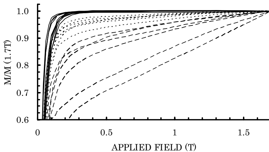
Fig. 5 Normalized IRM acquisition curves for Unzen samples in fields of up to 1.7 T. Solid, dotted, and broken lines denote type A, type B, and type C samples, respectively.
