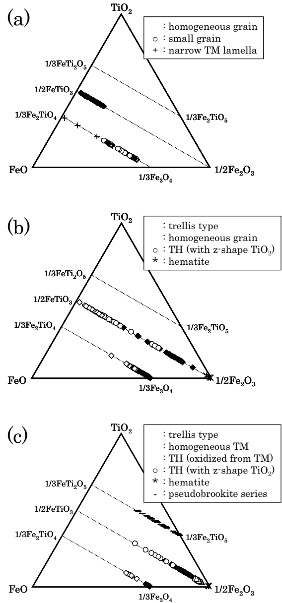
Fig. 9 \text{TiO}_2 - \text{FeO} - 1/2\text{Fe}_2\text{O}_3 ternary diagrams showing compositions of iron-titanium oxide minerals in Unzen samples: (a) type A, (b) type B, and (c) type C samples. Minor components allocated as follows: \text{FeO} = \Sigma\text{R}^{2+} = \text{Fe}^{2+} + \text{Mg} + \text{Mn} + \text{Ca} ; \text{Fe}_2\text{O}_3 = 1/2\Sigma\text{R}^{3+} = 1/2(\text{Fe}^{3+} + \text{Al} + \text{Cr}) ; \text{TiO}_2 = \Sigma\text{R}^{4+} = \text{Ti} + \text{Si} .
