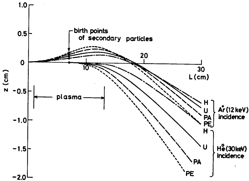
Fig. 3. Comparison of displacement in the toroidal direction for {}^4\text{He}^0(30\text{ keV}) atom and {}^{40}\text{Ar}^+(12\text{ keV}) ion incidence. Four types of plasma current profiles (H), (U), (PA) and (PE) are assumed.
