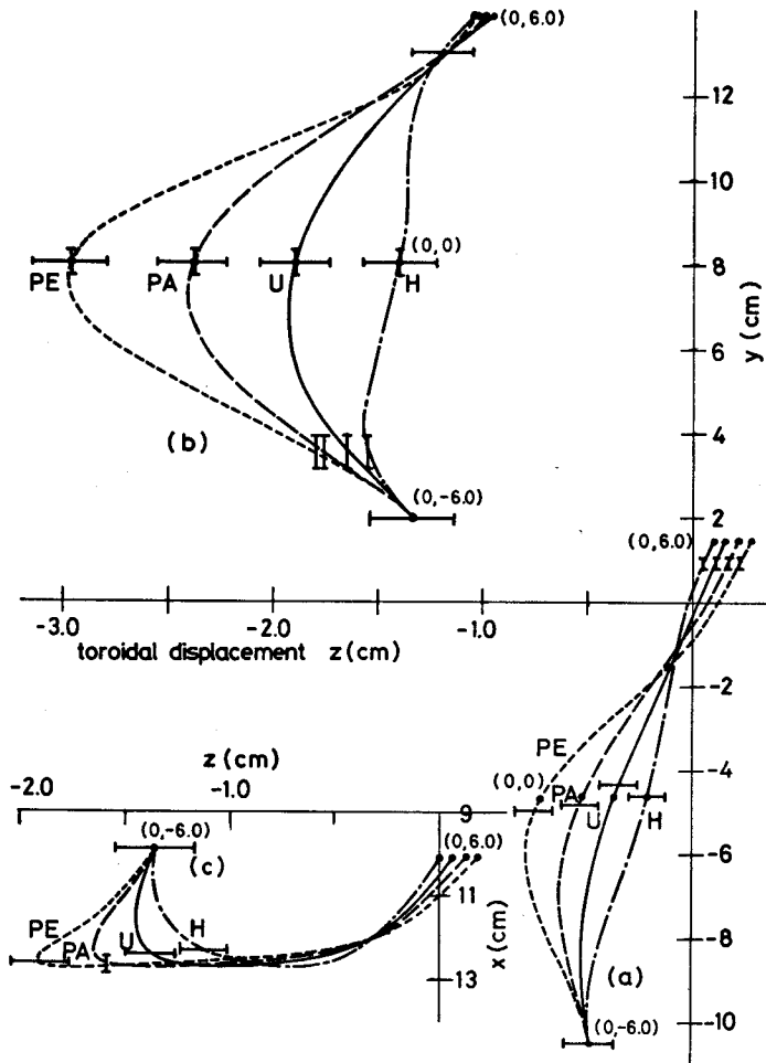
Fig. 4. Traces of secondary ions for four different current profiles (H) through (PE) at three different positions of detection (a), (b) and (c). Primary beam is of {}^4\text{He}^0 atoms (30 keV). Detector positions are (a) x = 6.5 cm and ions hit the plate on the plasma-side, (b) x = 6.5 cm but ions hit the opposite side, and (c) y = 1.5 cm. Bars show beam spread brought about by the incident beam divergence of \pm 5 mrad in z -direction and \pm 20 mrad in y -direction.
