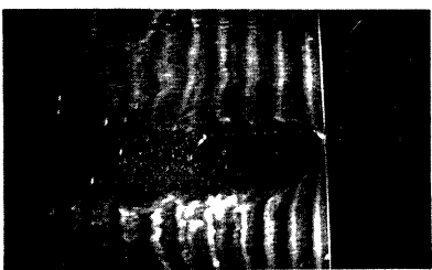
Photo. 5 Flow pattern (1:3 with Upper Deflector \alpha = 0^\circ )
