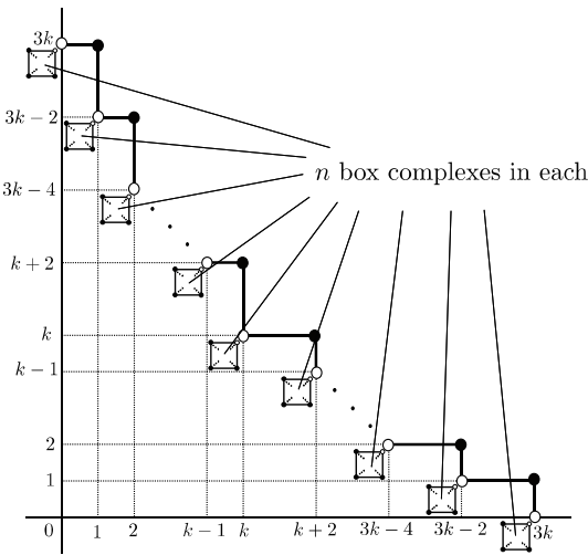
Figure 7: The complex \text{CFK}^\infty(K_n^{(3,3k+1)}) . This complex consists of the staircase complex, which is consistent with the complex of \text{CFK}^\infty(T(3,3k+1)) , and box complexes. The differential is represented by a line segment instead of an arrow, since the differential always lowers filtration levels.
