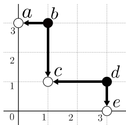
Figure 1: \text{CFK}^\infty(T(3,4)) . We can see that \partial b = a + c and \partial d = c + e .
