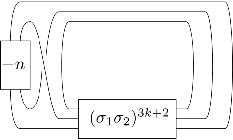
Figure 6: The case q = 3k + 2 ( k \geq 1 ). The box with -n contains n left handed vertical full-twists.
