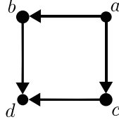
Figure 2: A box complex. The cycles are only d and b + c , but both are boundary cycles. Thus, it is an acyclic chain complex.
