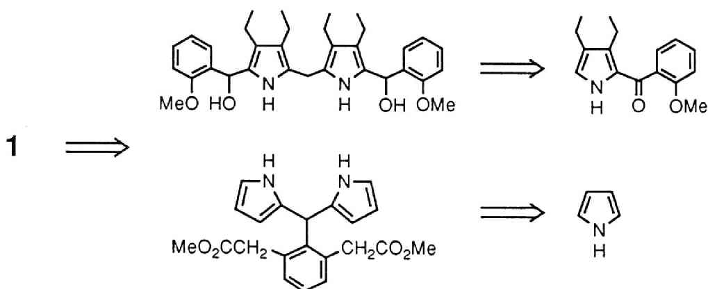
Scheme I. Retrosynthetic Analysis
