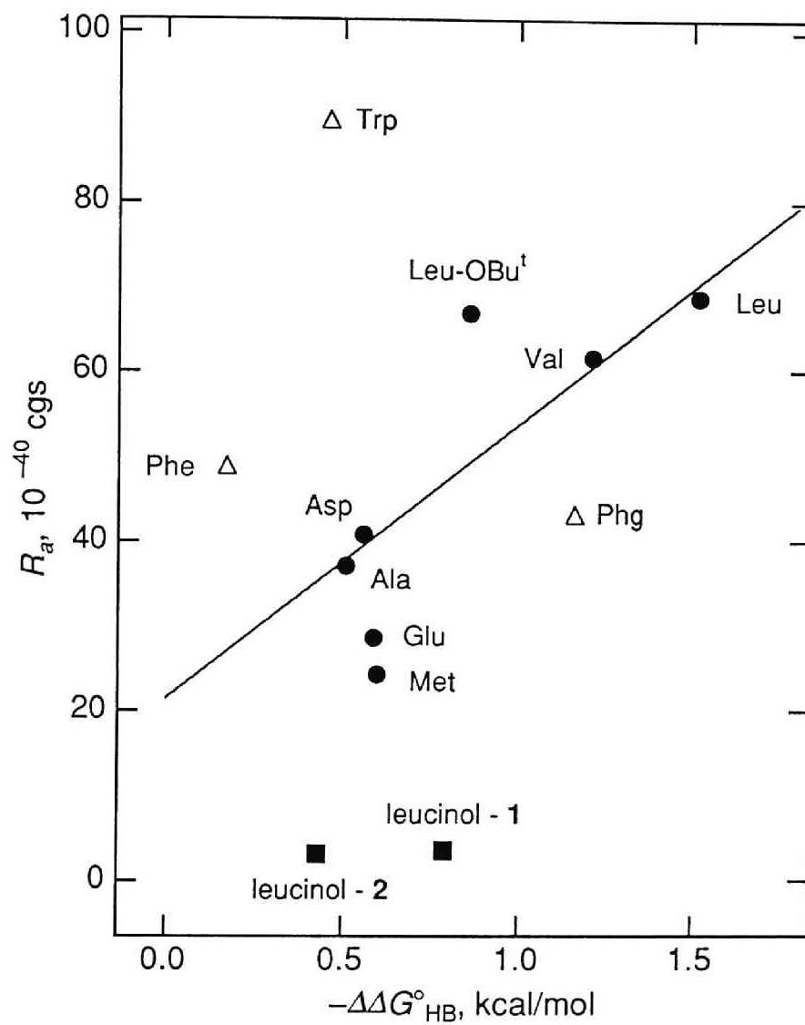
Figure 4. Plot of the rotational strengths( R_a ) against the hydrogen bonding energy( -\Delta\Delta G^\circ_{\text{HB}} ).
