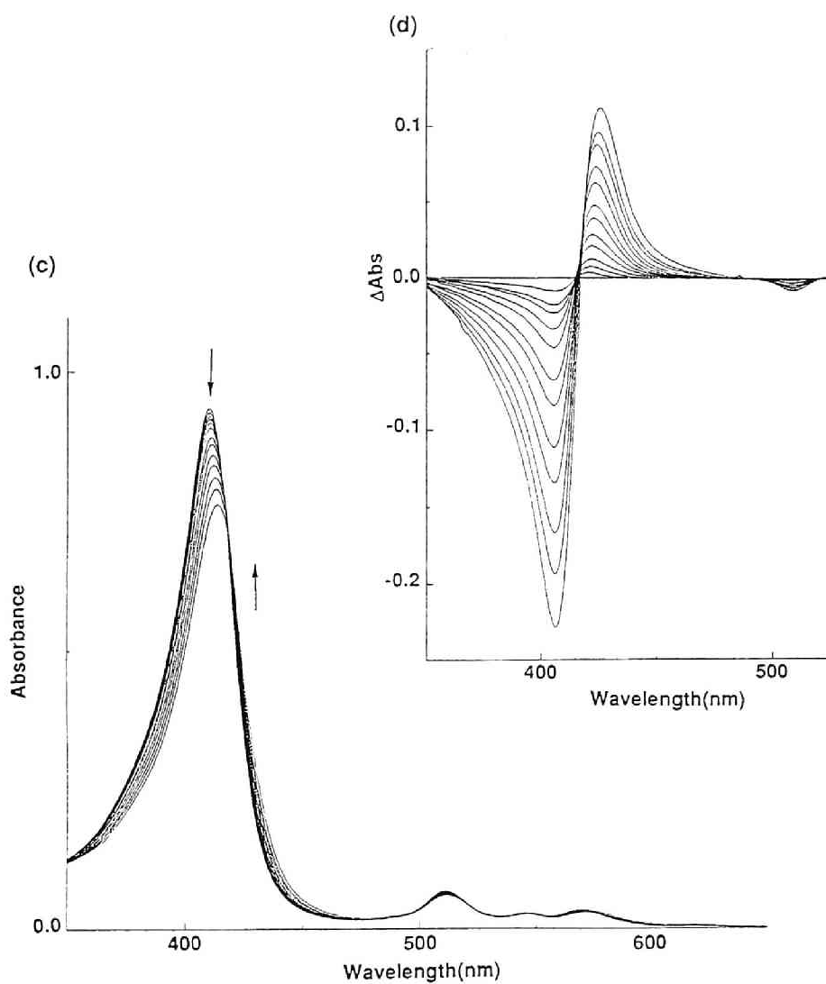
Figure 1. (c) Spectral change of 1 upon addition of 2 , 6-naphthalenedisulfonate ( G4 ) in 50 mM Tris buffer (pH 7.0) at 25 °C. (d) Difference spectra around the Soret region.
