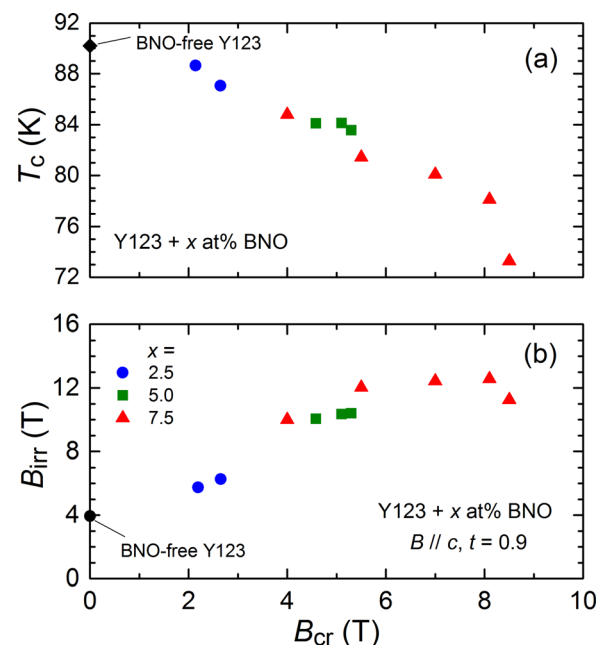
FIG. 5. B_{cr} dependences of (a) T_c and (b) B_{irr} at t = 0.9 for BNO-doped Y123 films with x = 0, 2.5, 5.0 , and 7.5 at. %, together with data of a BNO-free Y123 film ( T_s = 870 °C).
