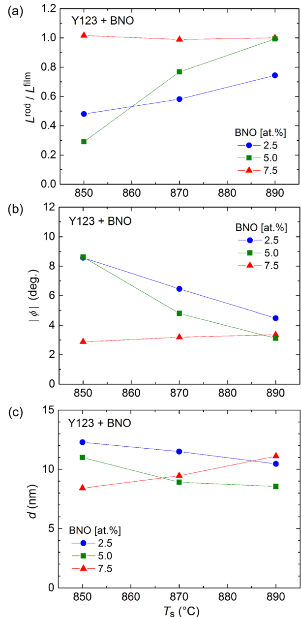
FIG. 3. Changes in mean values of (a) L_{\text{rod}}/L_{\text{film}} , (b) \phi , and (c) d of the BNO nanorods for BNO-doped Y123 films with T_s = 850, 870 , and 890^\circ\text{C} as a function of T_s .
