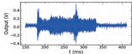
Fig. 2 Abrupt excitation of magnetic fluctuation. Fluctuation amplitude increases abruptly at 270 ms.
