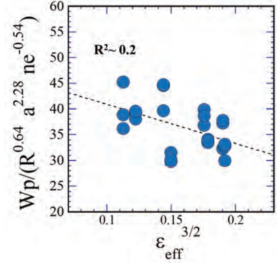
Fig. 4 Normalized stored energy W_p/R^{0.64}a^{2.28}n_e^{-0.54} against effective helical ripple \varepsilon_{\text{eff}} , indicating \varepsilon_{\text{eff}} is not a prominent explanatory variable of W_p values.
