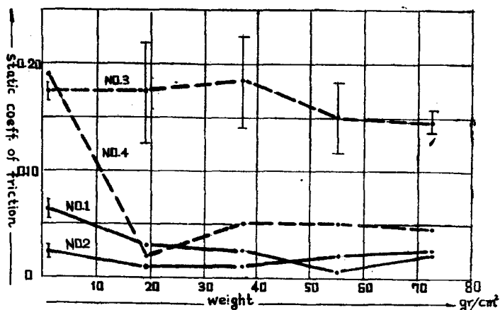
Fig. 1. Static coefficient of friction between 20% gelatine-jelly and a polished glass surface, when supplied with mobile oil as lubricant.
