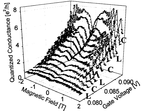
FIG. 3. Magnetoconductance in low magnetic field for various gate voltages. Mark "L" and "C" indicate a Lorentzian type and a cusp-like type, respectively.
